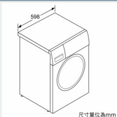
Dimensioned drawings
