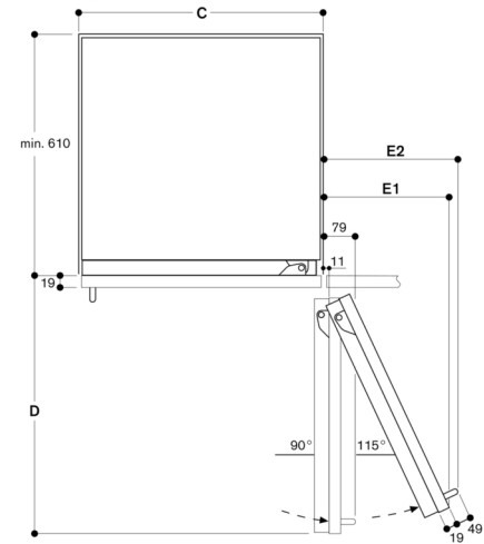
Veggavstand RB 472/RC/RF/RW
