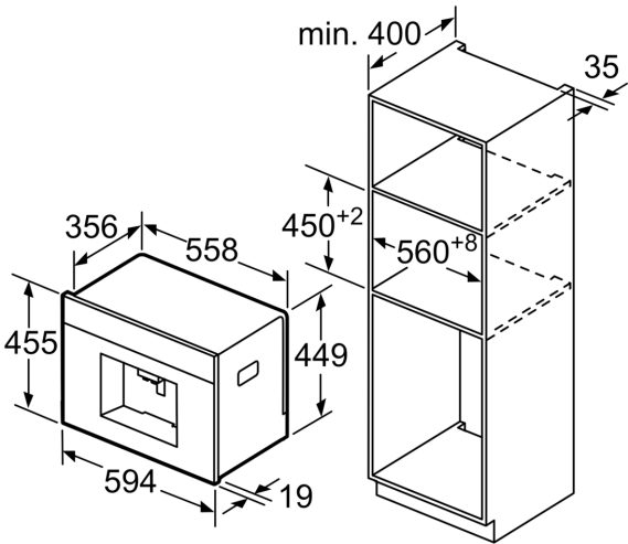
Bean and water containers are removed from the front. Recommended installation height 95-145 cm.
