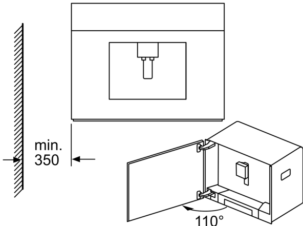
If using the 92° hinge limiter (spare part no. 00636455), the minimum distance to the wall is only 100 mm.
