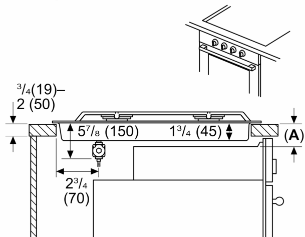
Measurements in inches (mm) Cooktop over oven
