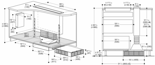
A: Surface mounting B: Flush mounting C: 29 1/2\"/>
