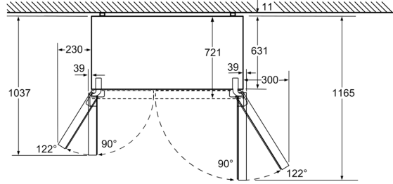
Chilling drawers can be pulled out completely at a door opening angle of 122° measurements in mm
