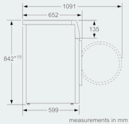
Dimensioned drawings
