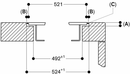
Cross-section
