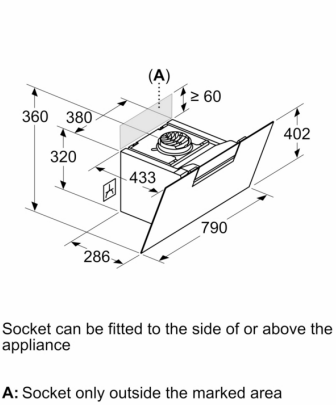
Measurements in mm Appliance in circulated air mode without duct
