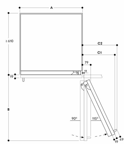
Wandabstand RVB/RVC/RVF/RVW
