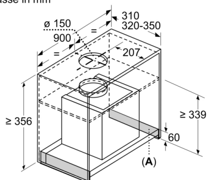
Masse in mm
