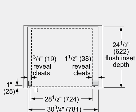
Flush Install Top View
