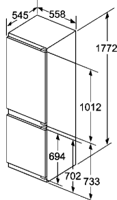
KI42FP60/GI38NP60 (Fridge Left Hinged/Freezer Right Hinged)
