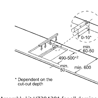
Assembly kit HZ394301 for all domino hobs
