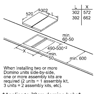
*Applies to 30cm domino hobs*
