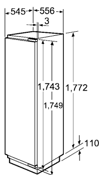
KI42FP60/GI38NP60 (Fridge Left Hinged/Freezer Right Hinged)
