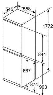
KI42FP60/GI38NP60 (Fridge Left Hinged/Freezer Right Hinged)
