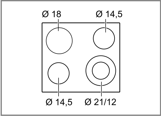
ET6..HN17., ET6...BNA1.
