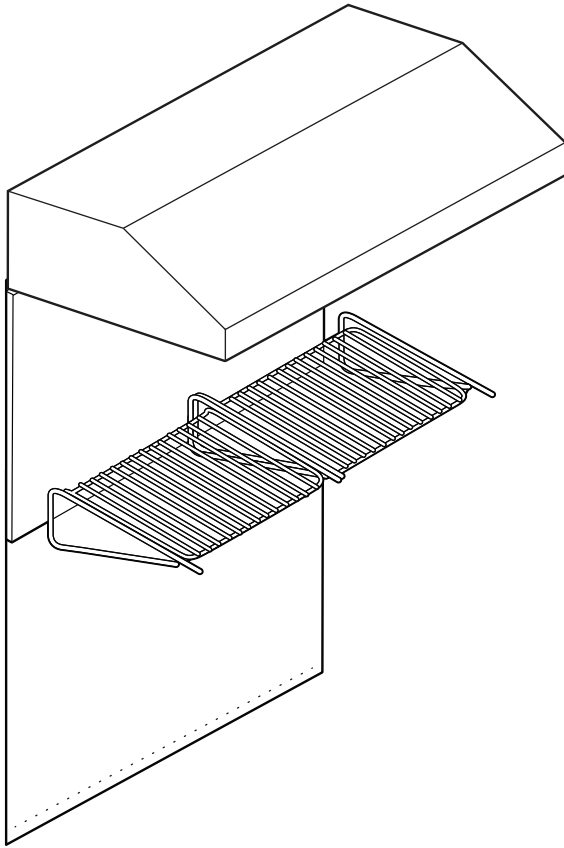
Figure 10: Backsplash with a Keep Hot Shelf
