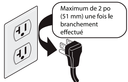
Figure 5 : Connexion murale
