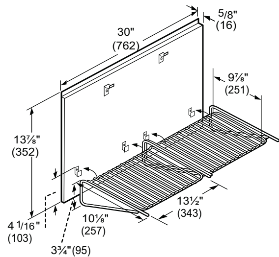
Figure 12: Keep Hot Shelf
