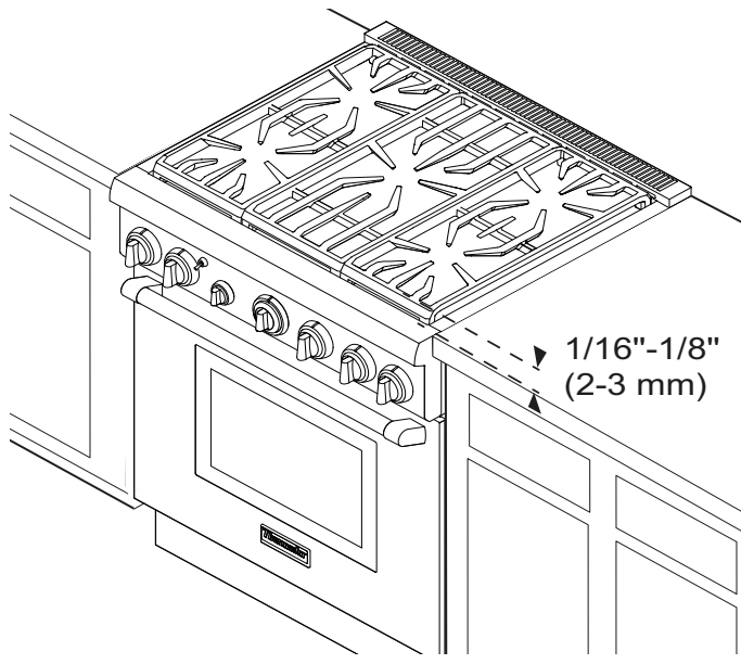
Figure 22: Adjusting the Height of the Range
