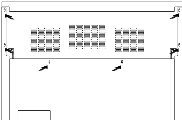
Figure 15: Zero Clearance Trim Rear Screw Removal
