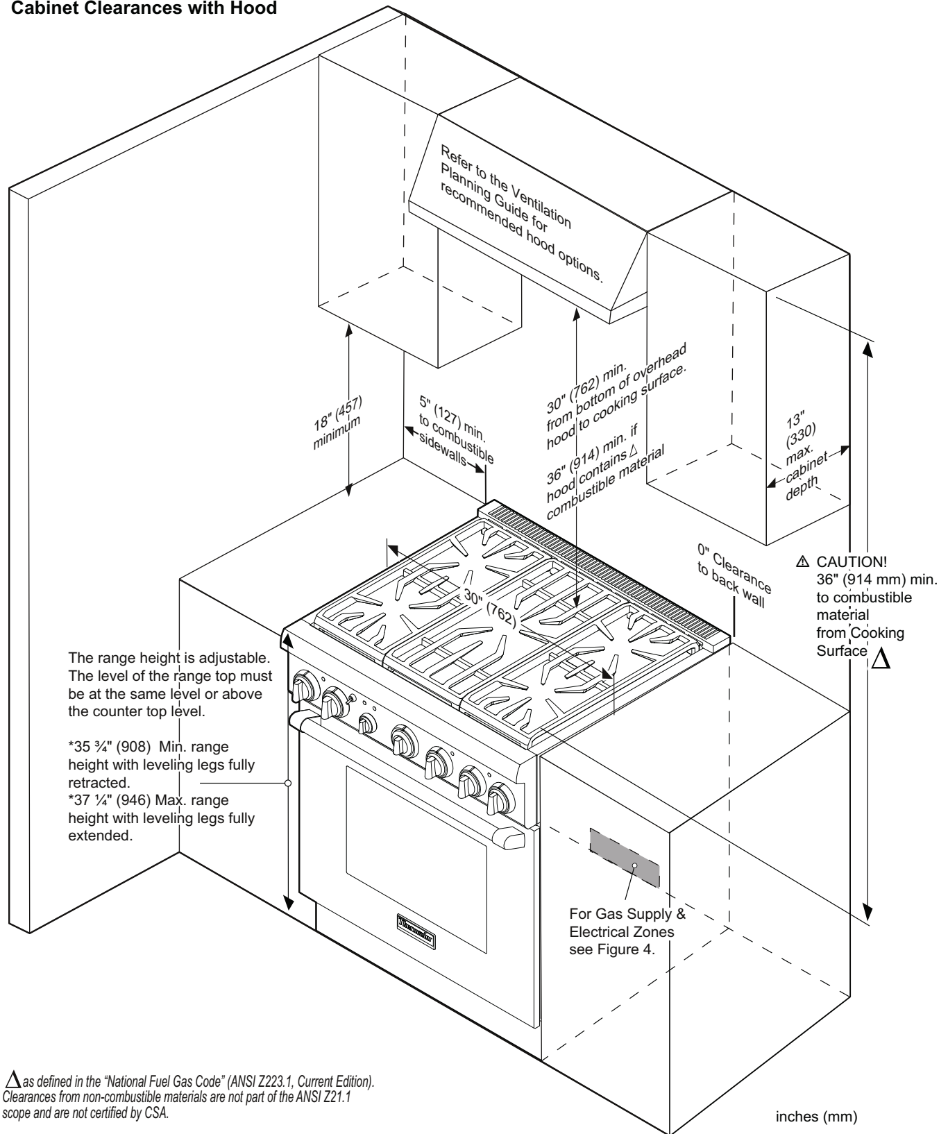
Figure 1: Cabinet Clearances
