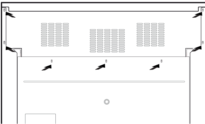
Figure 19: Zero Clearance Trim Rear Screw Removal
