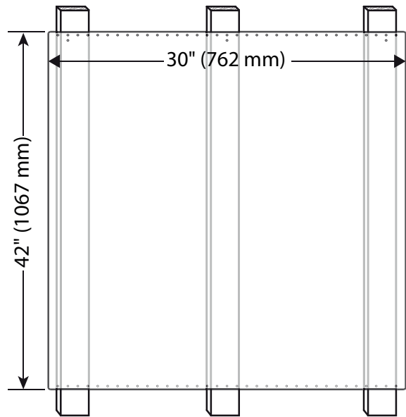
Figure 13: Backsplash Installation
