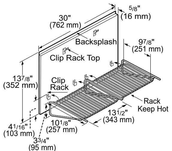
Figure 16: Keep Hot Shelf
