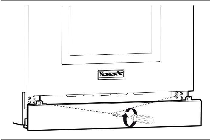
Figure 27: Kick Panel Adjustment
