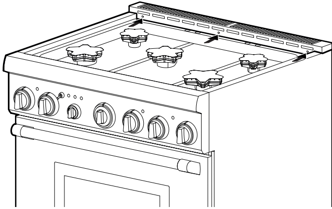
Figure 18: Zero Clearance Trim Front Face Screw Removal
