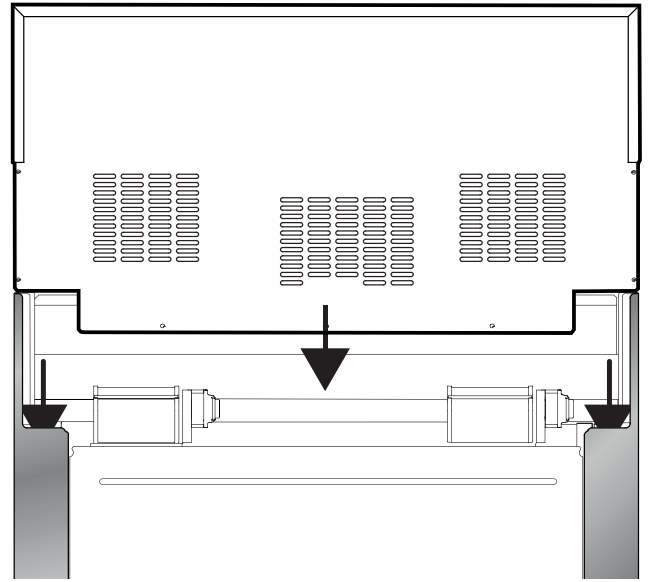
Figure 20: Backguard Installation
