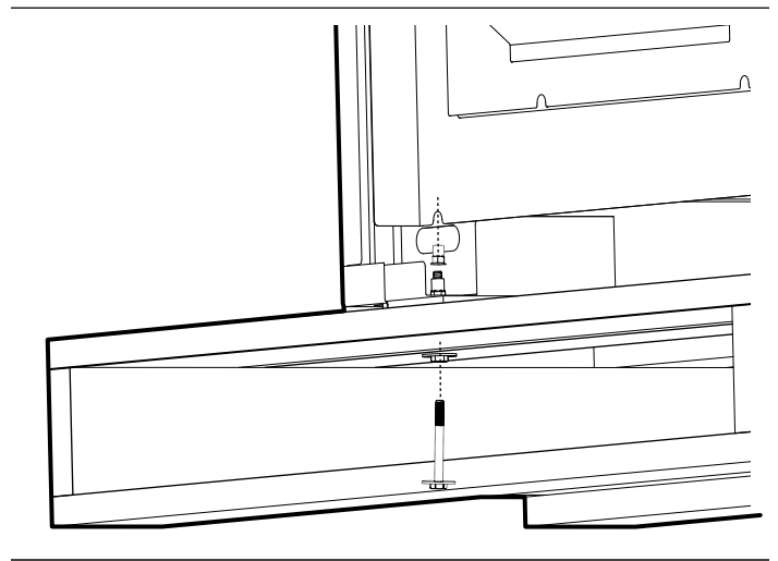
Figure 6: Removal of Shipping Bolts
