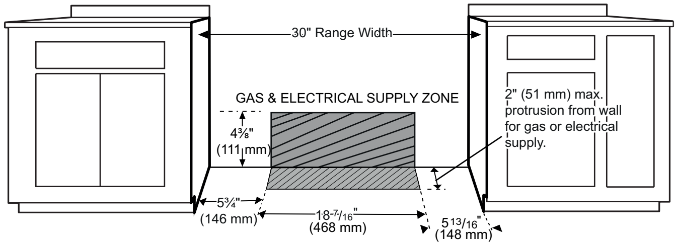
Figure 4: Gas & Electrical Supply Locations
