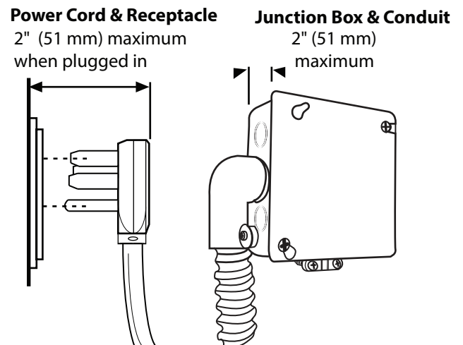
Figure 5: Wall Connection
