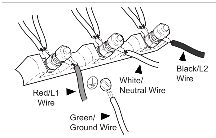
Figure 10: 4-Wire Connection
