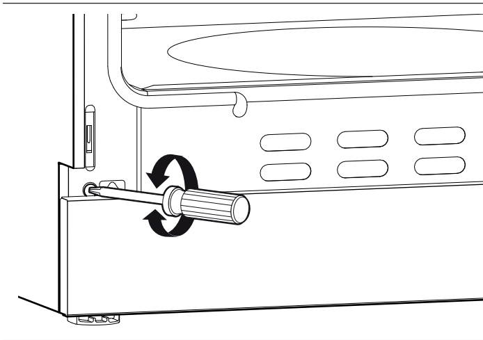
Figure 24: Hinge Receiver Adjustment Screw
