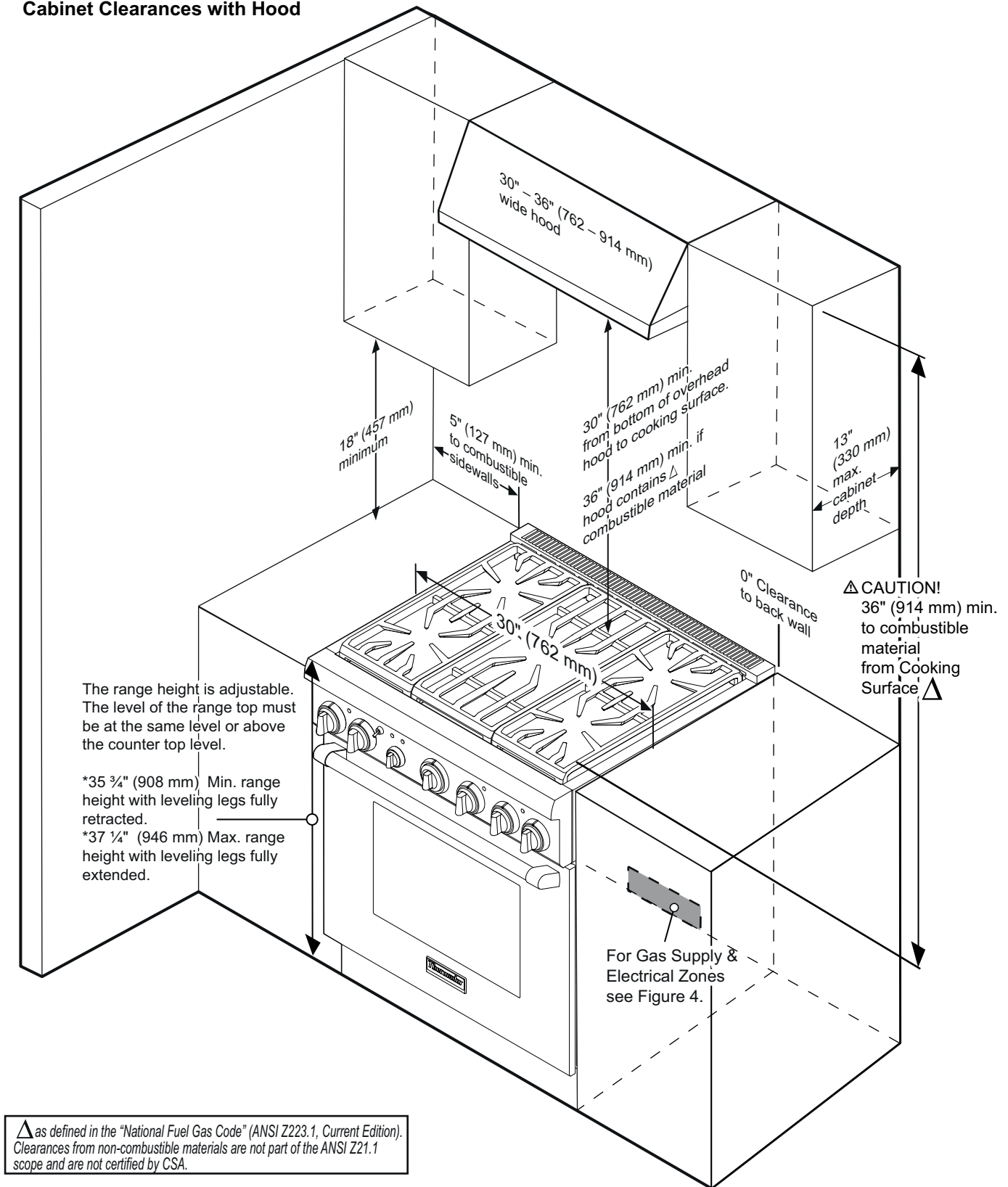
Figure 1: Cabinet Clearances with a Hood
