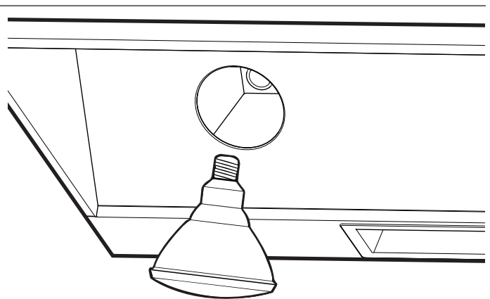
Figure 8: Heat Lamp Replacement
