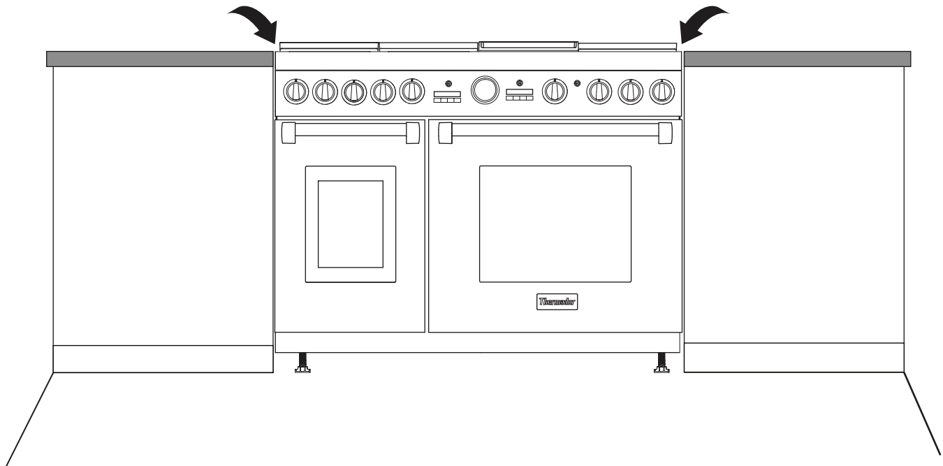
Figure 31: Adjusting the Height of the Range
