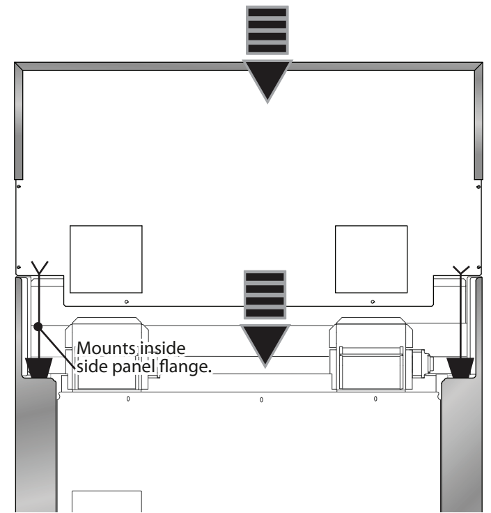
Figure 29: Backguard Installation
