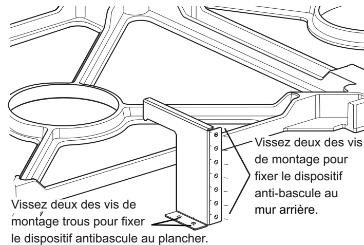
Figure 14 : Support anti-bascule
