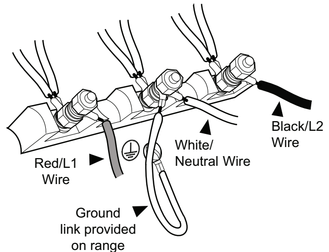
Figure 19: 3-Wire Connection
