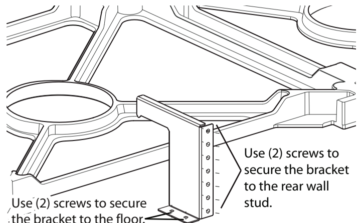
Figure 14: Anti-tip Bracket
