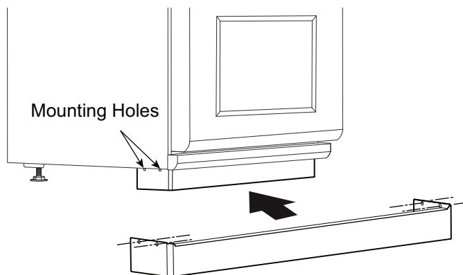
Figure 36: Toe Kick Panel Installation
