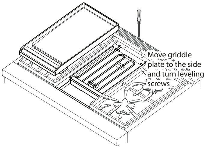
Figure 32: Griddle Leveling Screws
