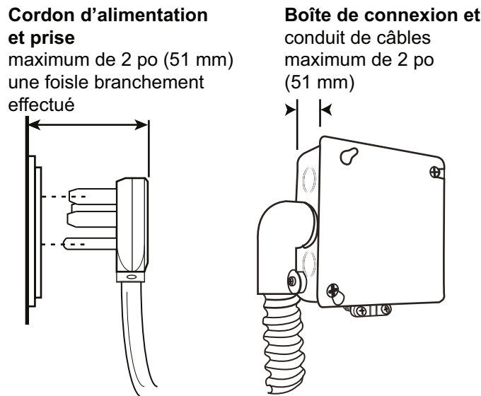
Figure 5 : Connexion murale
