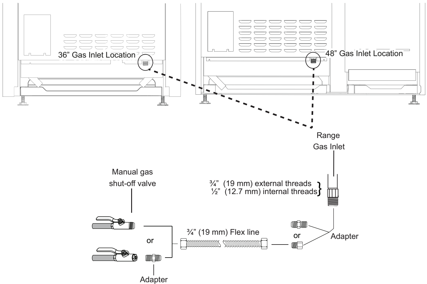
Figure 15: Gas Supply Connection
