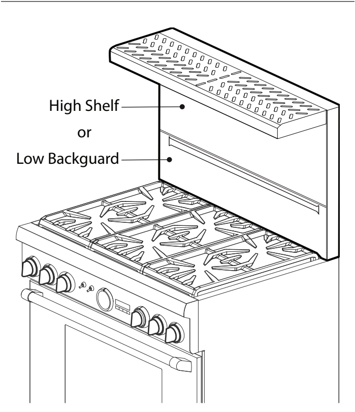
Figure 25: High Shelf & Low Back Front View
