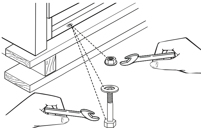
Figure 7: Removal of Shipping Bolts
