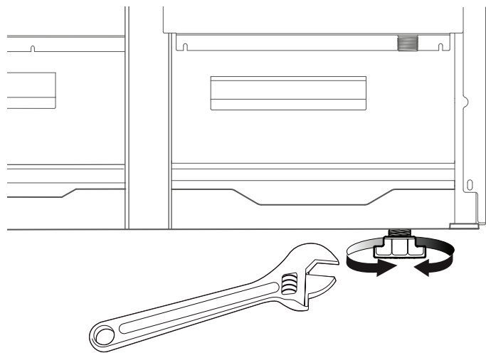
Figure 30: Leveling Legs
