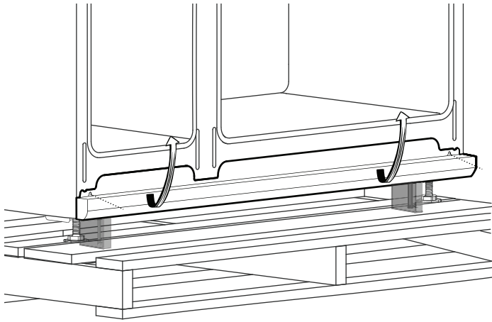
Figure 6: Door Trim Removal
