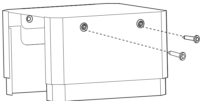
Figure 35: Leg Cover Mounting Holes
