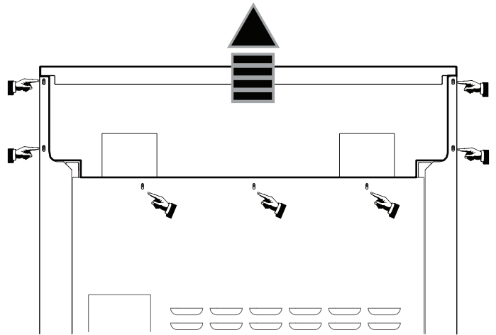
Figure 28: Flush Island Trim Rear Screw Removal
