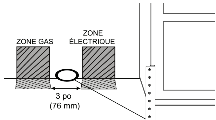
Figure 13 : Emplacement du support anti-bascule
