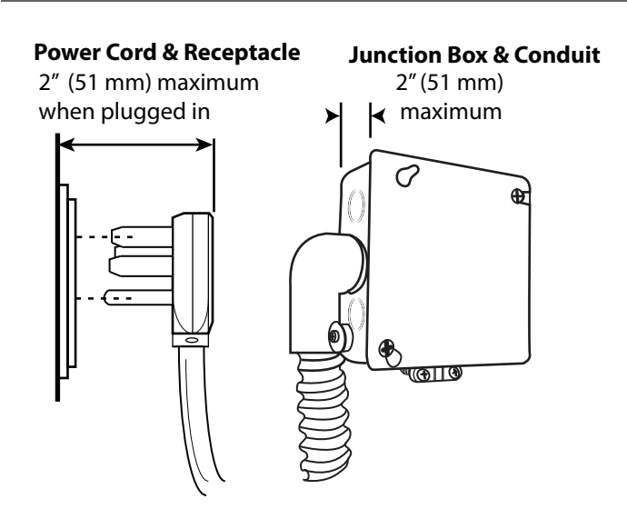
Figure 5: Wall Connection
