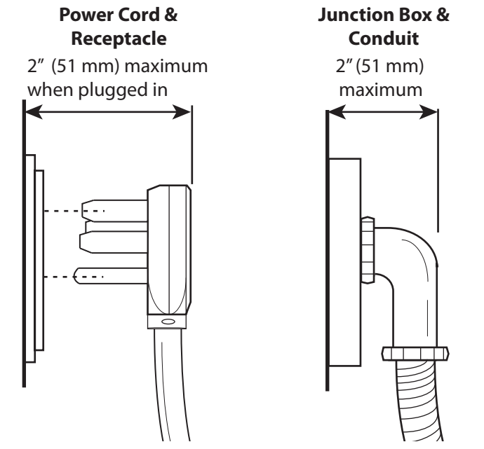
Figure 5: Wall Connection
