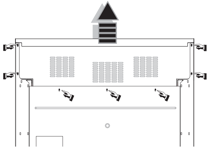
Figure 23: Flush Island Trim Rear Screw Removal
