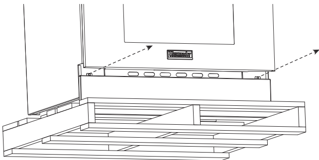
Figure 6: Remove Kick Panel
