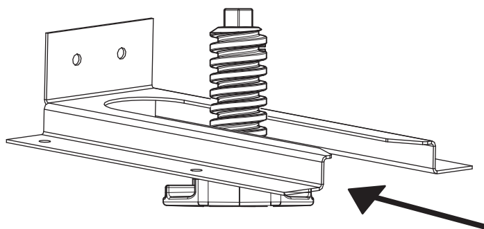
Figure 9: Anti-Tip Bracket
