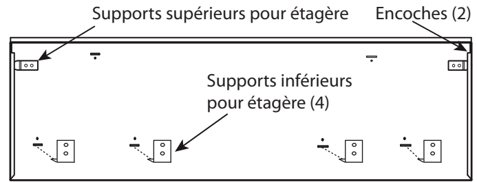
Figure 19 : Dos de la plaque murale
