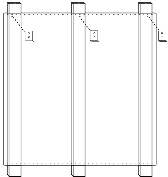
Figure 17: Backsplash with a Keep Hot Shelf
