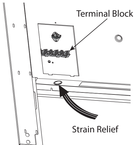
Figure 13: Strain Relief Location
