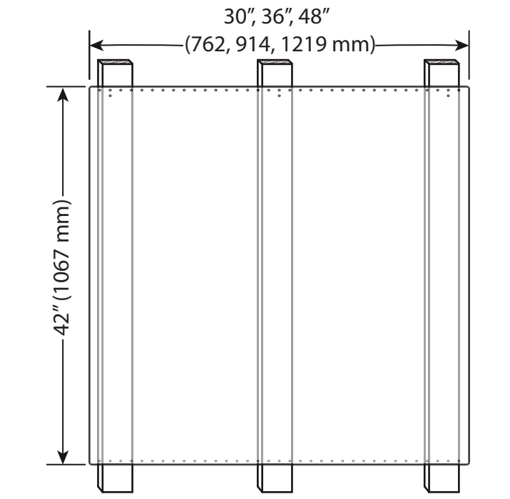
Figure 15: Backsplash Installation
