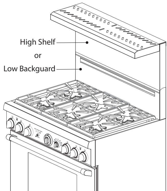
Figure 20: High Shelf & Low Back Front View
