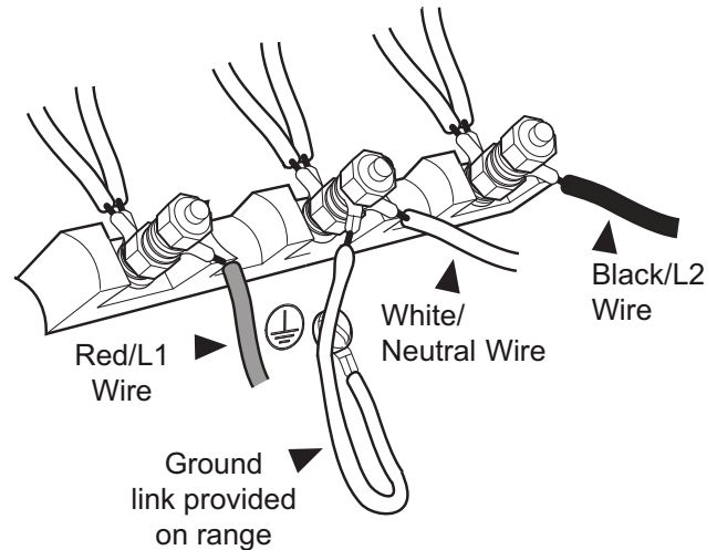
Figure 14: 3-Wire Connection
