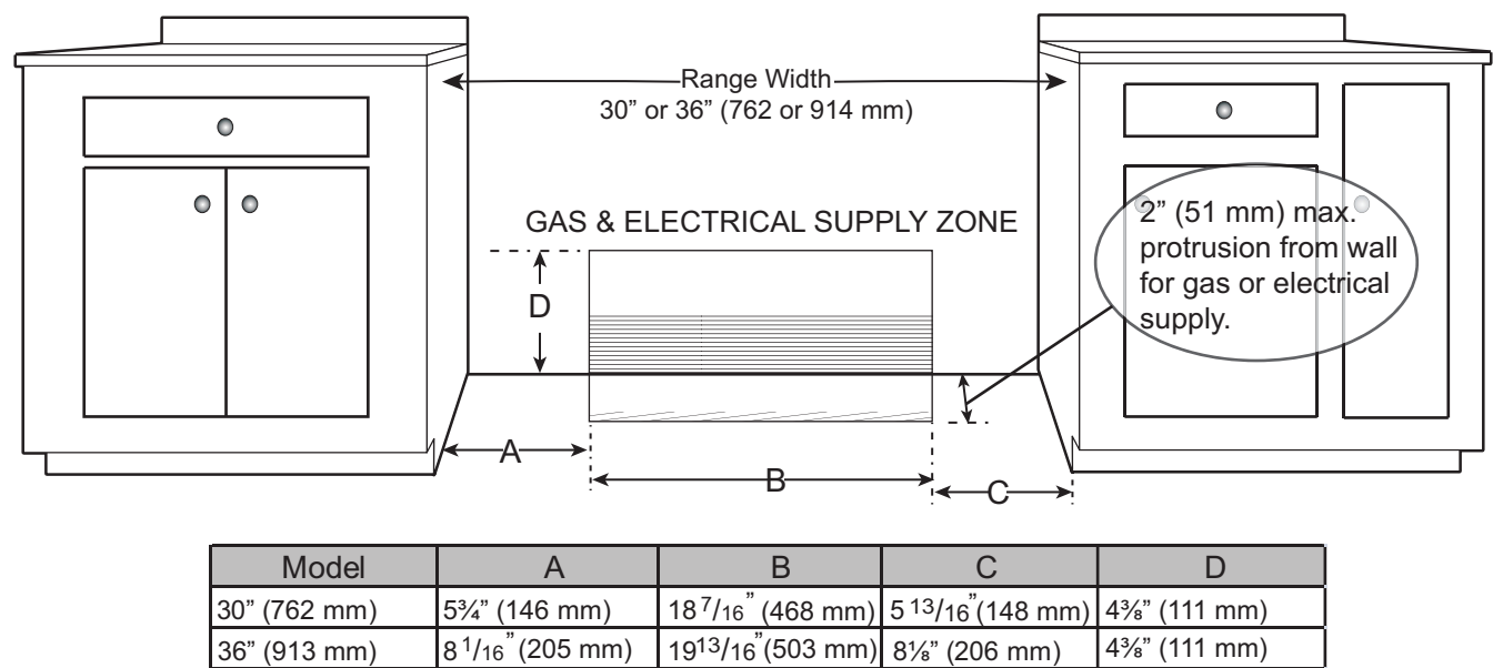
Gas & Electrical Supply Locations for 30" and 36" Dual Fuel Ranges
