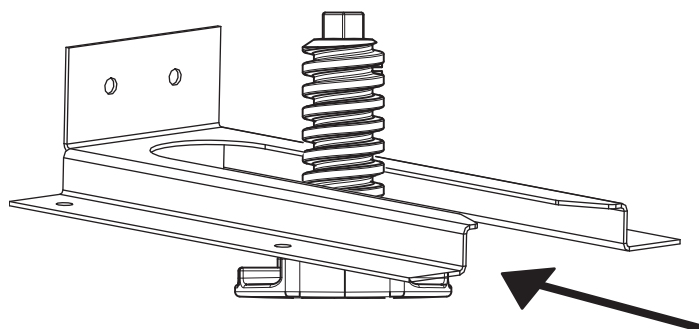
Figure 9 : Patte antibascul
