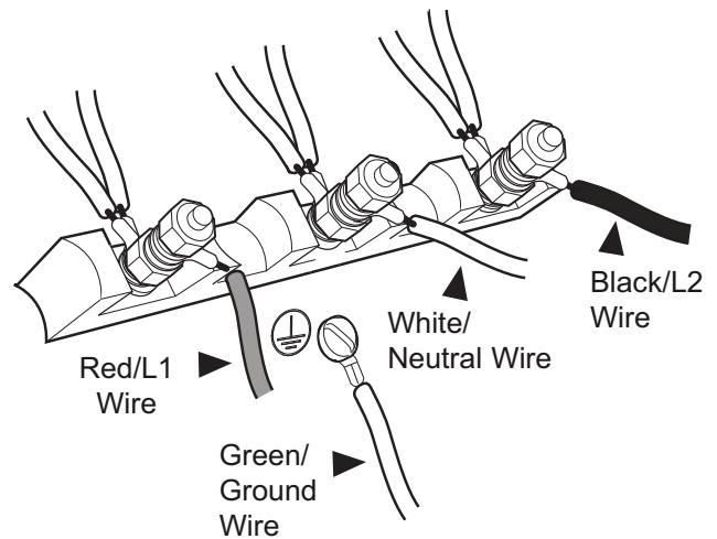
Figure 12: 4-Wire Connection
