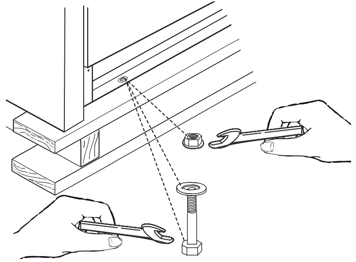
Figure 7: Removal of the Shipping Bolts
