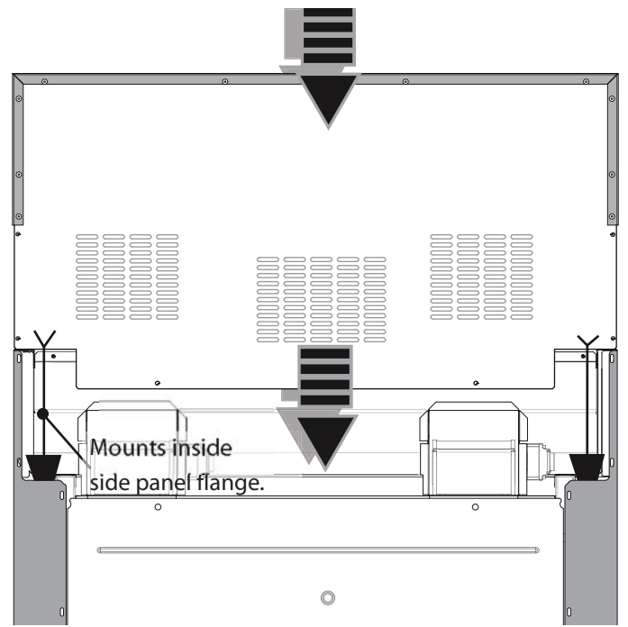
Figure 24: Backguard Installation
