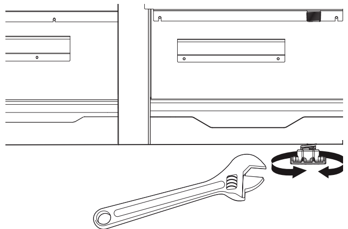
Figure 29: Leveling Legs
