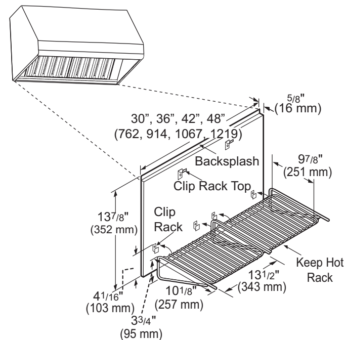
Figure 18: Keep Hot Shelf
