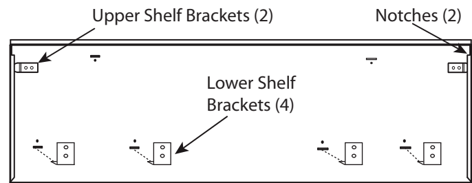
Figure 19: 48" Back of Wall Plate
