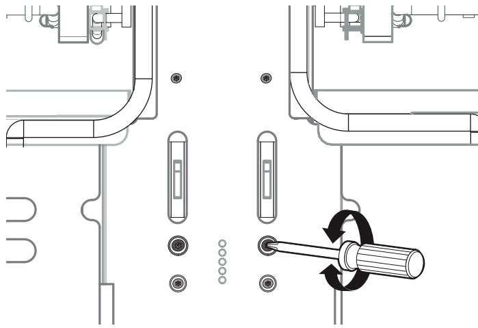
Figure 27: Hinge Receiver Adjustment Screw
