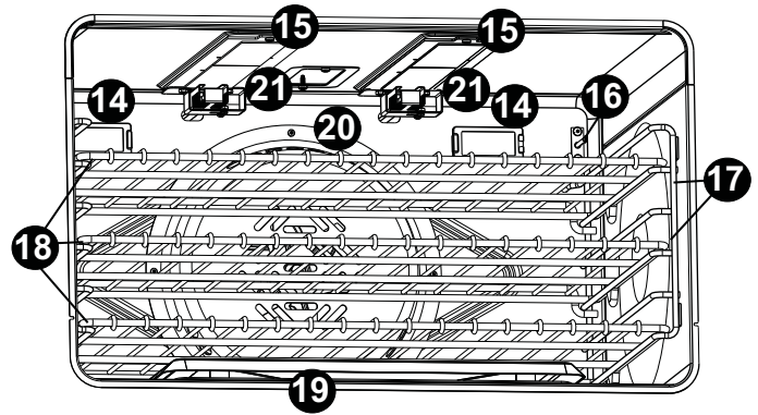
Figure 5: Gas Oven Interior
