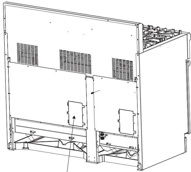
Figure 10: Location of Junction Box on 48" Ranges
