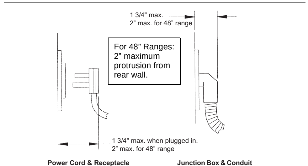
Figure 3b: Wall Connection
