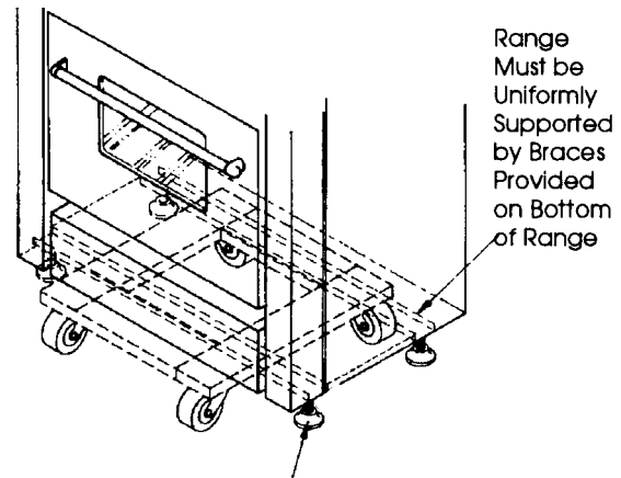
FIG. 5- Dolly Positioning
