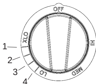
ExtraLow Settings
