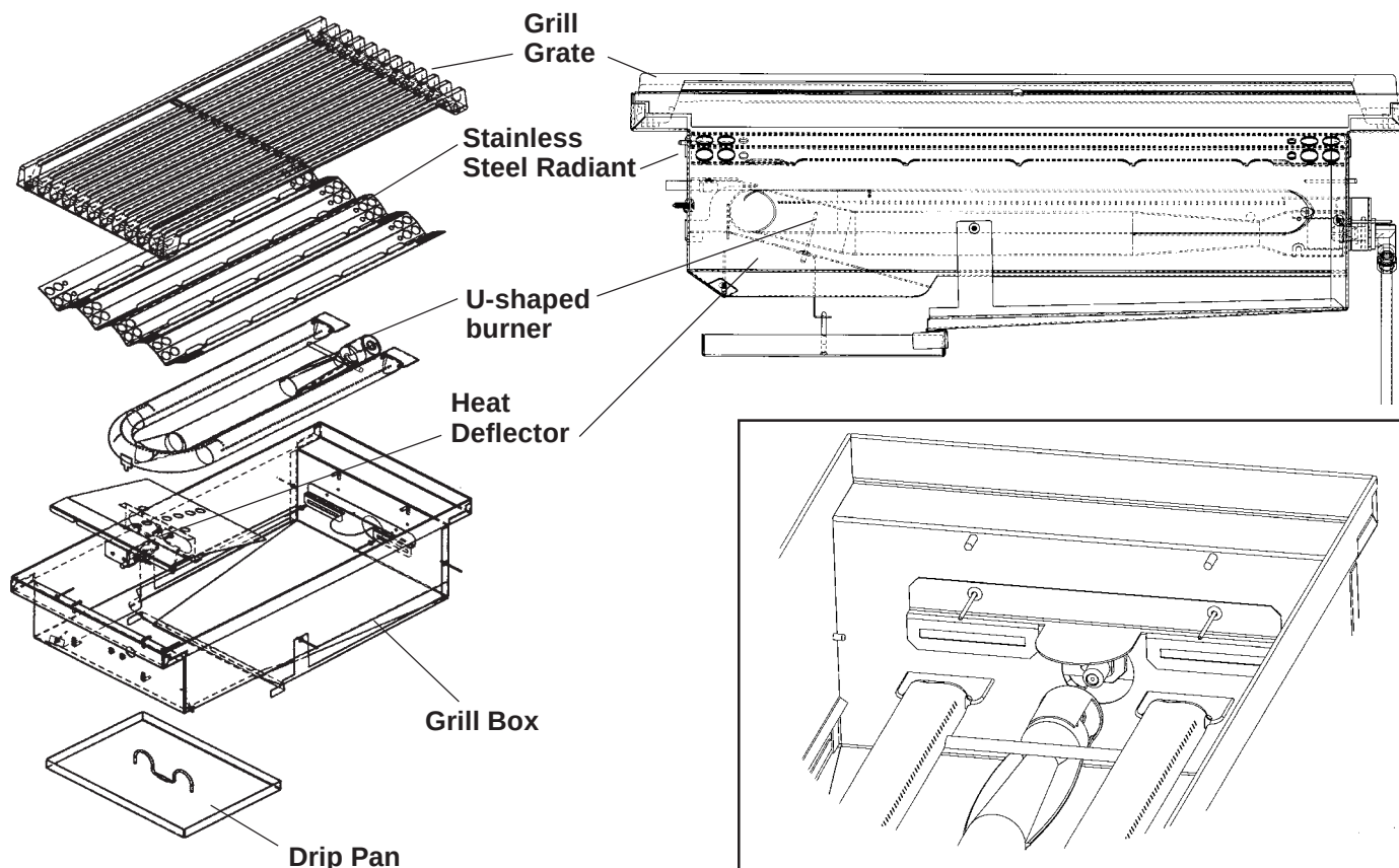
Burner Placement in slots in back of grill
