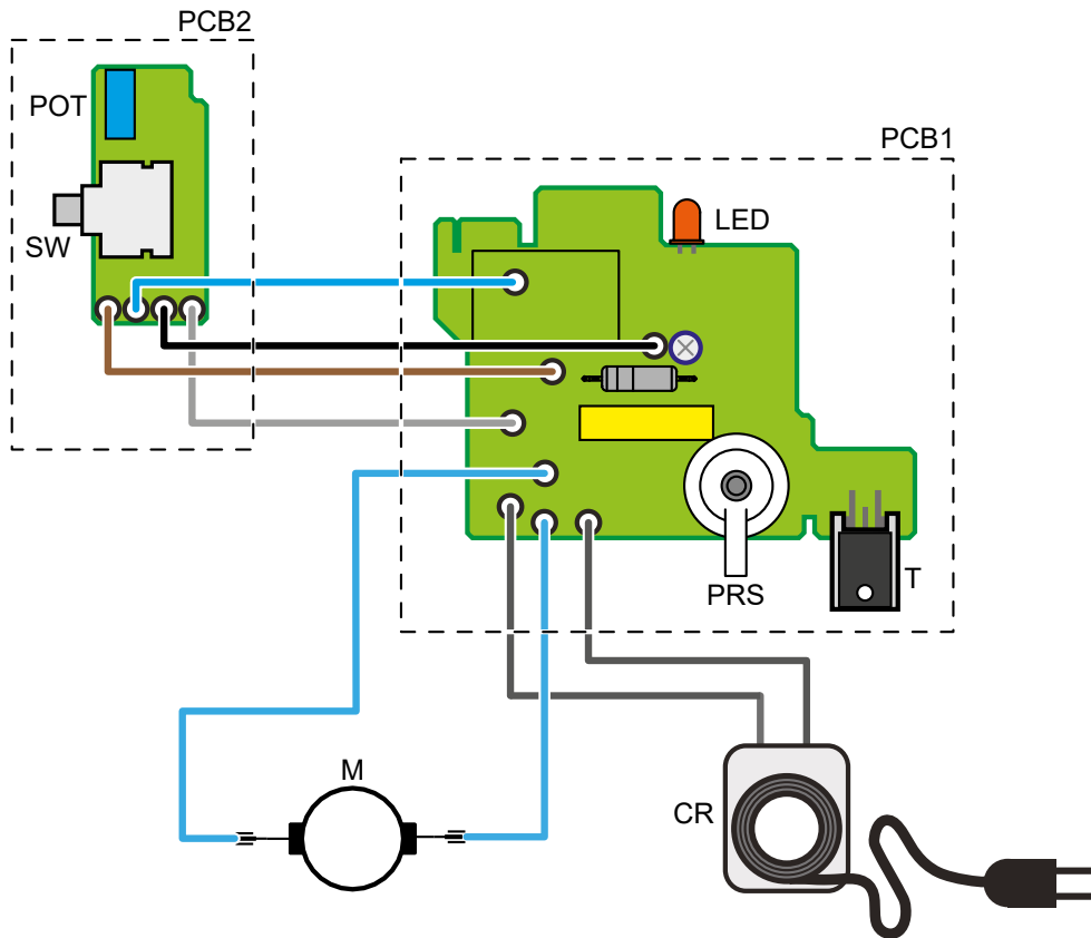
Fig. 1: Connection diagram
