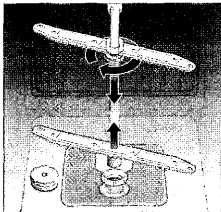
Spray arms
