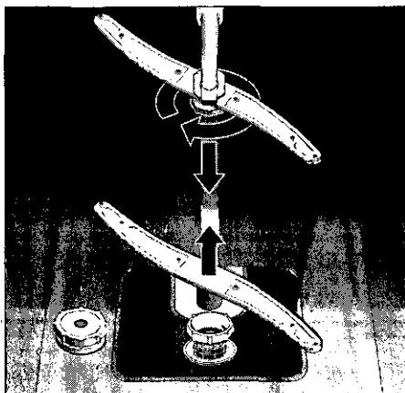
Spray arms
