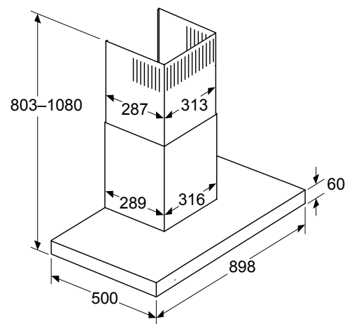
Recirculation operation
