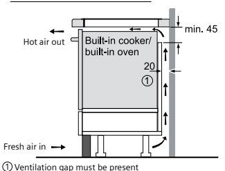
Induction hob over an oven
