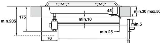
For connection using flexible gas tubing
