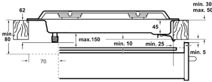
For connection using flexible gas tubing
