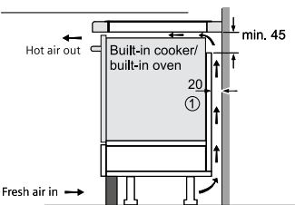
Induction hob over an oven
