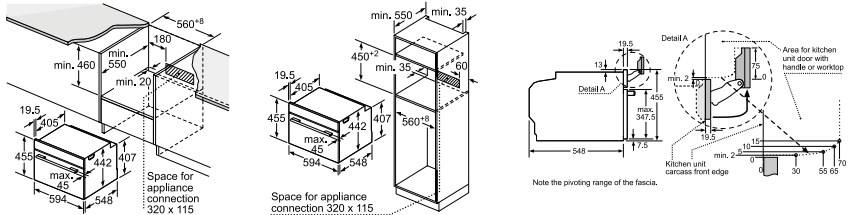
Installation with a hob.
