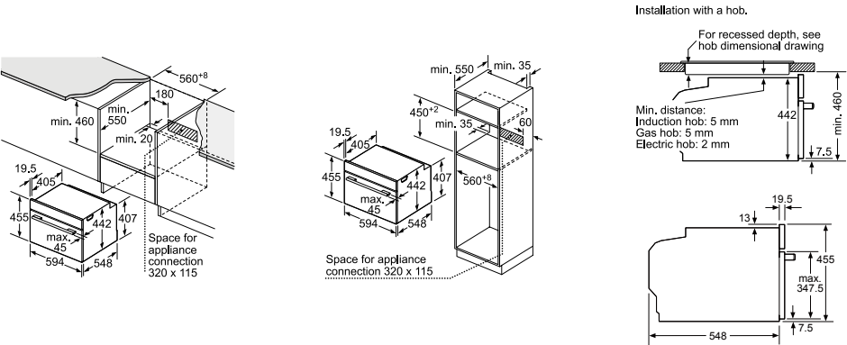
Installation with a hob.
