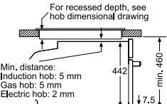
Installation with a hob.
