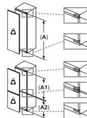
Recommended gap dimensions for flat hinges
