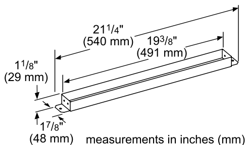
HDDSTRAN2 Transition for Rectangular Duct for Downdraft
