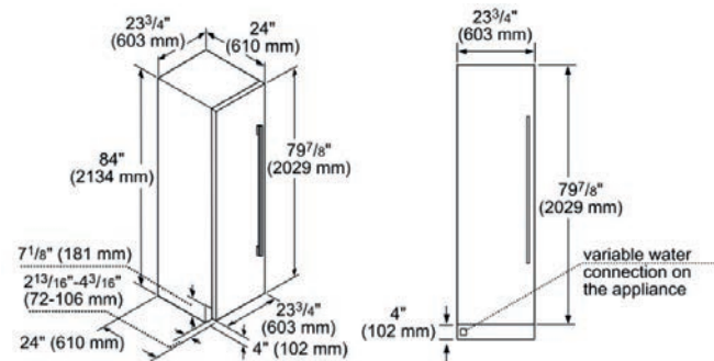
iQ700 Freezer with fixed hinge 60.3 cm FI24NP33
