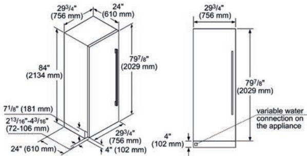
iQ700 Freezer with fixed hinge 75.6 cm FI30NP33
