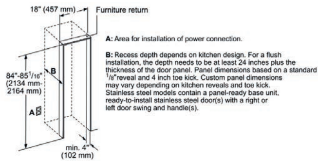
iQ700 Wine cabinet with glass door 45.1 cm CI18WP03
