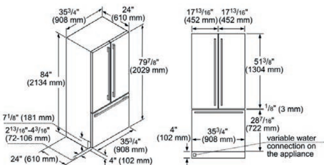
iQ700 Fridge with bottom freezer 90.8 cm CI36TP02
