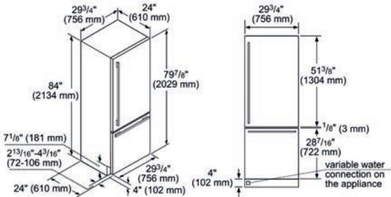
iQ700 Fridge with bottom freezer 75.6 cm CI30BP02
