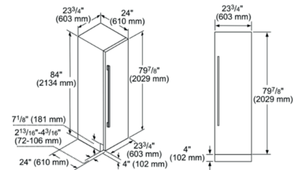
iQ700 Fridge with fixed hinge 60.3 cm CI24RP02
