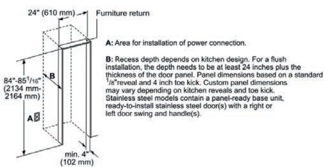
iQ700 Wine cabinet with glass door 60.3 cm CI24WP03
