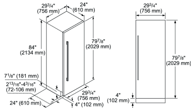
iQ700 Fridge with fixed hinge 75.6 cm CI30RP02
