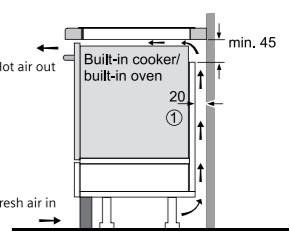
Induction hob over an oven
