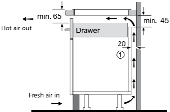
Induction hob over a drawer
