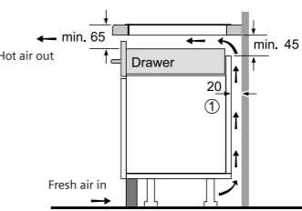
Induction hob over a drawer
