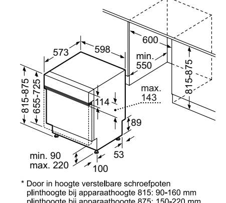
SN5... Maten in mm
