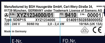
Example of a rating plate
