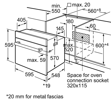
*20 mm for metal fascias Measurements in mm
