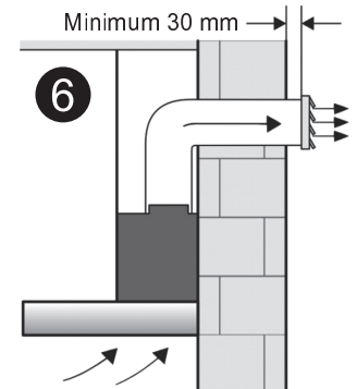
Connect outside the wall
