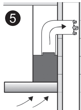
Connect to common flue
