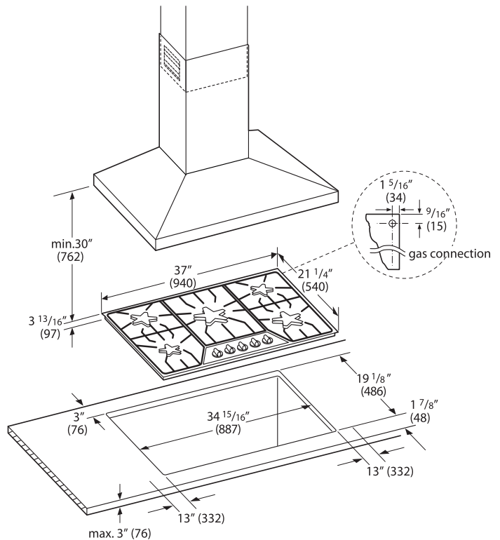
Figure 2: Cutout Dimensions
